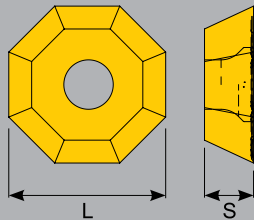
OFKT 05T3
